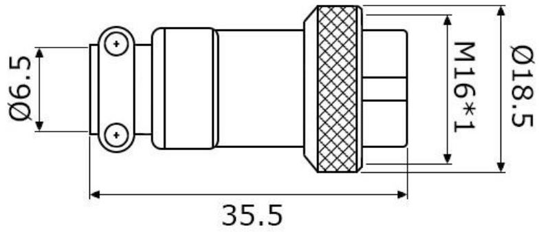
SZC-CONNECTOR
